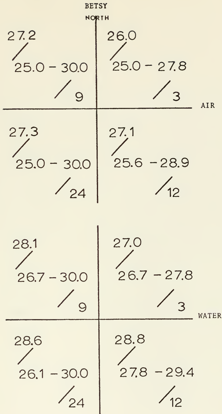
Figure 12. Air and Sea-Surface Observed Temperature Data by Quadrant for Hurricane Betsy -- 080000GMT SEP - 100000GMT SEP 1965. (MEAN/RANGE OF OBSERVATIONS/NO. OF OBSERVATIONS)
